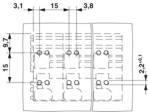
Drilling diagram
